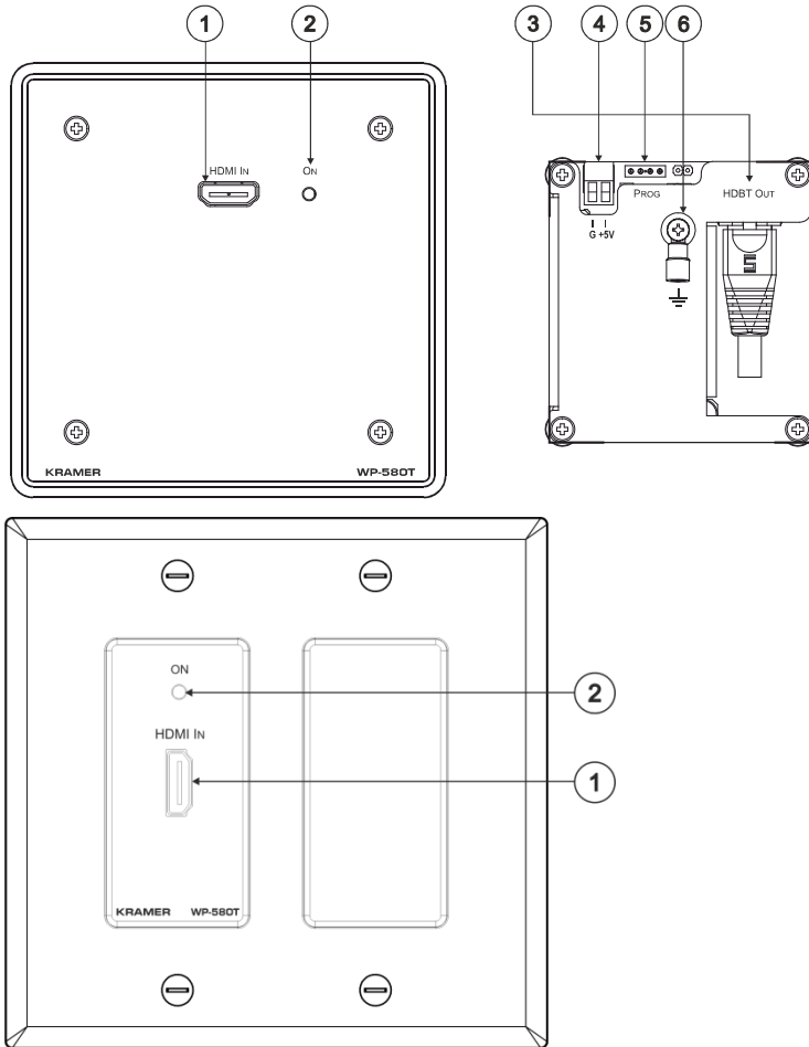
Figure 1: WP-580T HDMI Line Transmitter for the US and US-D Sizes
