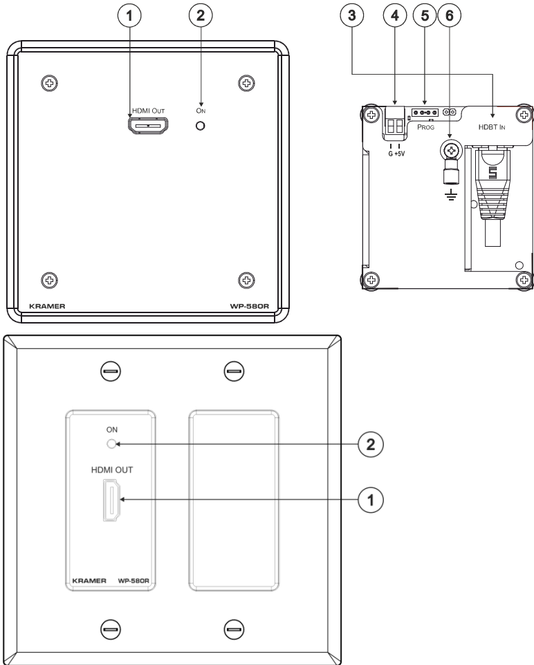
Figure 3: WP-580R HDMI Line Receiver for the US and US-D Sizes
