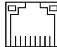
LAN: pin view of panel connector
