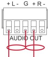
Figure 7: Connecting the Balanced Output to an Unbalanced Stereo Audio Acceptor
